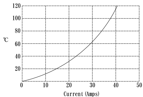
Mating UJMPT20AG with UJMST20AG (Page 13A2)
