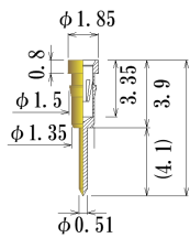
J0010-GG-ST (Value type)
