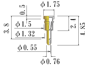
Acceptable plug: \phi 0.60 \sim \phi 0.40 JS0041-1L-GG
