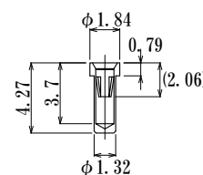
JS0020-GG-634 (J-634contact, High force)
