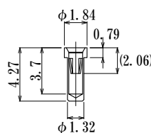
JS0020-GG-ST (JV11contact, value type)
