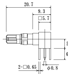
Plug DM537P75-PC-L1
