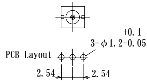
Plug DM537P-PC-L2
