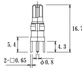
Plug DM537P75-PC
