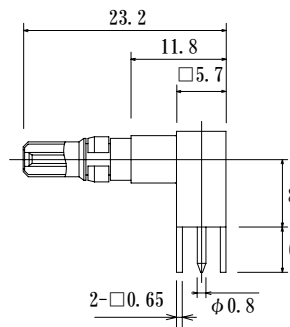
Plug DM537P75-PC-L2
