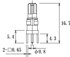
Plug DM537P-PC
