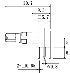
Plug DM537P-PC-L1
