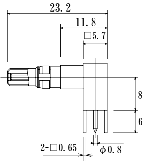
Plug DM537P-PC-L2
